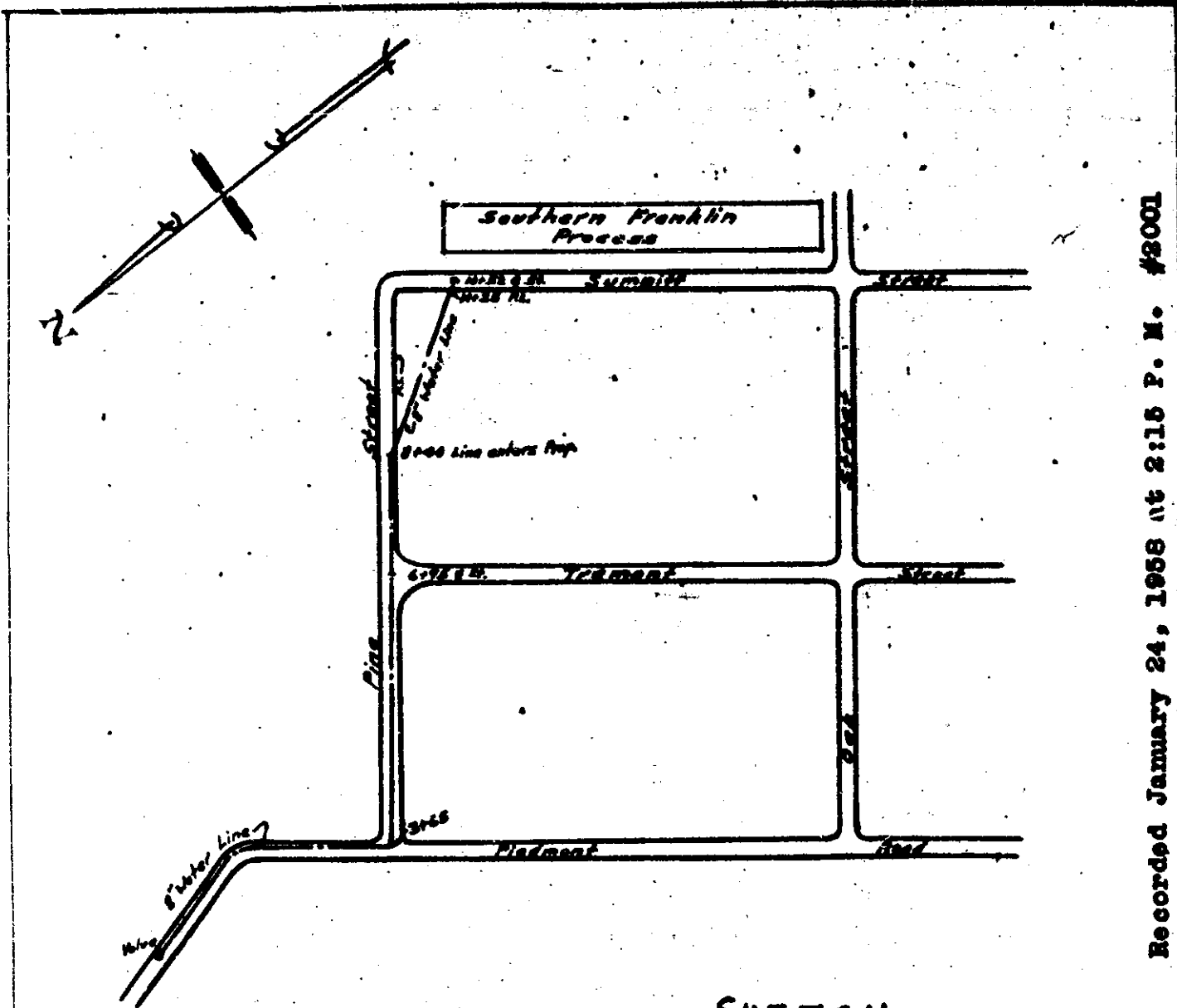
SKETCH SHOWING 8" WATER LINE SOUTHERN FRANKLIN PROCESS CO. GREENVILLE, S.C.
